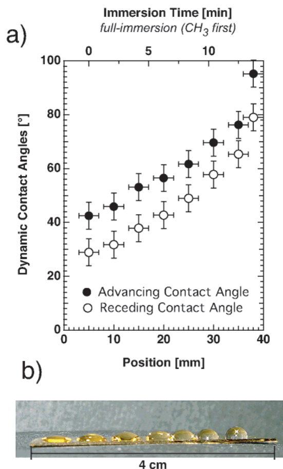
Figure 2. (a) Dynamic contact angles along a hydrophobicity gradient using full-immersion ( \text{CH}_3 -first) as the preparation method. The small hysteresis of less than 15^\circ between the advancing and the receding contact angles is an indication for the formation of a full monolayer. (b) Water droplets along a hydrophobicity gradient using full-immersion ( \text{CH}_3 -first) as the preparation method.
